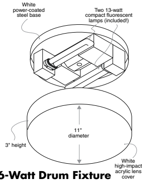
26-Watt Drum Fixture
